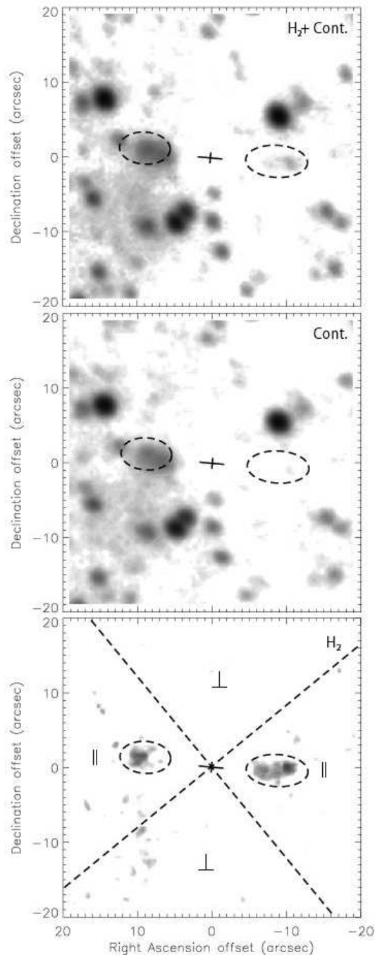
Figure 1. G320.23-0.28 (IRAS 15061-5814) H 2 +continuum, continuum, and residual H 2 images. The cross represents the maser group location with the elongated axis showing the position angle of linear maser distribution. Dashed ellipses encompass areas of H 2 emission. Dashed lines in the H 2 image divide the frame into quadrants parallel and perpendicular to the maser position angle.
