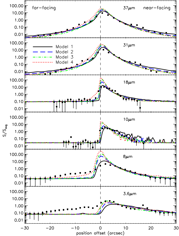
FIG. 4.— Intensity profiles along the outflow axis. The squares are observational data sampled at intervals of the resolutions of the instruments (intervals of 2 & 3 \times resolution are used for 18 & 10 \mu\text{m} ) with errors composed of systematic flux uncertainties (assumed to be 20%) and estimated background noise. The lines are model profiles.
