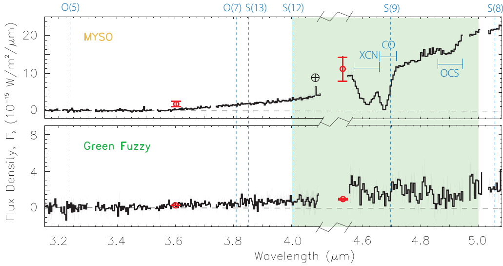
FIG. 4.— Combined L and M band spectra for G49.27-0.34. The light green area delineates the passband of the IRAC 4.5 \mu\text{m} filter. The only detectable emission features from the putative green fuzzy area is continuum emission. The expected lines of shock excited \text{H}_2 , which are delineated by vertical dashed blue lines with the transitions labeled at the top. Areas of the spectra with missing data were removed because of poor sky subtraction. In some cases bad pixels create false features which are delineated by the encircled cross symbol. Flux densities derived from the IRAC image photometry of the MYSO and the putative green fuzzy are plotted as red circles. No data are present from 4.10 to 4.55 \mu\text{m} where the atmosphere is opaque.
