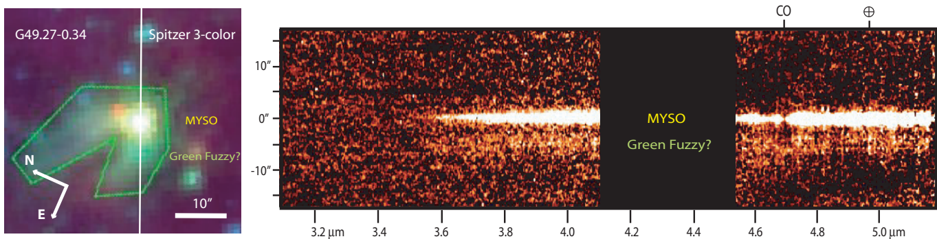
FIG. 2.— Green fuzzy emission from G49.27-0.34. (Left) A 3-color composite image from Cyganowski et al. (2008), with 3.6 \mu\text{m} as blue, 4.5 \mu\text{m} as green, and 8.0 \mu\text{m} as red. The area containing extended green emission is encompassed in the green contour. The NIRS slit position and angle used for spectroscopy is shown by the white line. (Right) 2-D images of the combined L and M band spectra (with 3-pixel smoothing for display purposes only) are shown with the same vertical spatial scaling as the figure on the left. The only detectable emission from the extended “green” emission area is continuum. The absorption feature of CO is marked, as well as a region that results from poor sky subtraction (encircled cross symbol). No data are present from 4.10 to 4.55 \mu\text{m} where the atmosphere is opaque.
