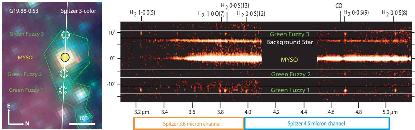
FIG. 1.— Green fuzzy emission from G19.88-0.53. (Left) A 3-color composite image from Cyganowski et al. (2008), with 3.6 \mu\text{m} as blue, 4.5 \mu\text{m} as green, and 8.0 \mu\text{m} as red. The area containing extended green emission is encompassed in the green contour. The NIRS slit position and angle used for spectroscopy is shown by the white line. (Right) 2-D images of the combined L and M band spectra (with 3-pixel smoothing for display purposes only) are shown with the same vertical spatial scaling as the figure on the left. White lines encompass the spectra of the three green fuzzy knots detected. The bandpasses of the IRAC 3.6 and 4.5 \mu\text{m} filters are shown at the bottom. The only detectable emission from the three green fuzzies are lines of shock excited H 2 , which are labeled at the top. The absorption feature of CO is also marked. No data are present from 4.10 to 4.55 \mu\text{m} where the atmosphere is opaque.
