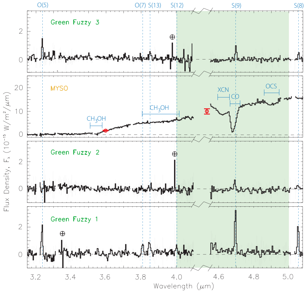
FIG. 3.— Combined L and M band spectra extracted from the locations within G19.88-0.53 marked as circles in Figure 1. The light green area delineates the passband of the IRAC 4.5 \mu\text{m} filter. The only detectable emission features from the three green fuzzies are lines of shock excited \text{H}_2 , which are delineated by vertical dashed blue lines with the transitions labeled at the top. Areas of the spectra with missing data were removed because of poor sky subtraction. In some cases bad pixels create false features which are delineated by the encircled cross symbol. Flux densities derived from the IRAC image photometry of the MYSO are plotted as red circles. No data are present from 4.10 to 4.55 \mu\text{m} where the atmosphere is opaque.
