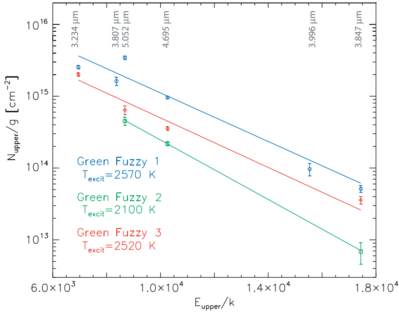
FIG. 5.— Excitation diagram of the \text{H}_2 level column density distribution towards the green fuzzy knots in G19.88-0.53. We are able to fit these data with single temperatures value for each of the green fuzzy knots (solid lines).
