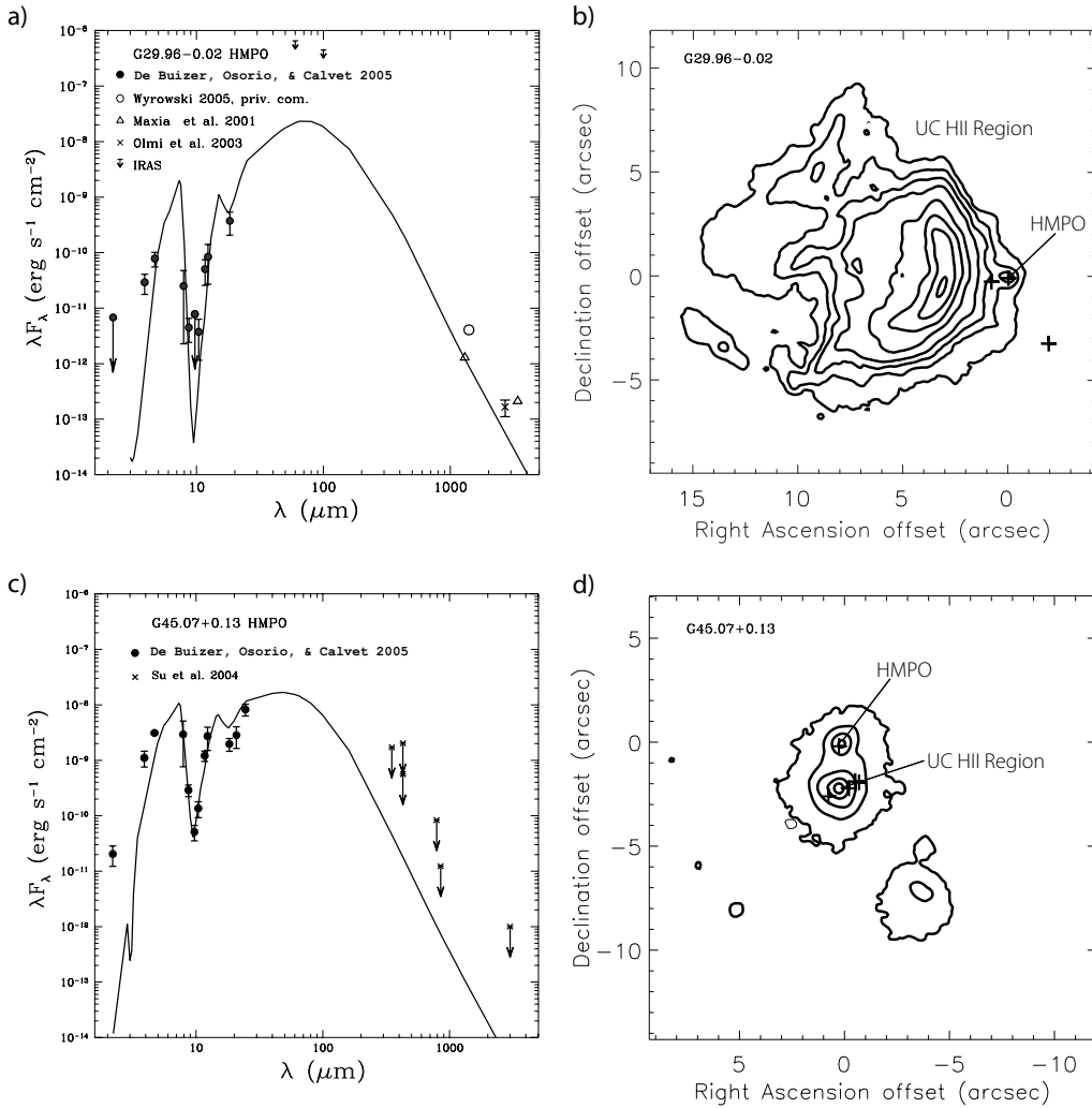
Figure 1. (a) Observed and model SEDs for the G29.96-0.02 HMPO. The different symbols represent the observed values of the flux densities from the references indicated. Error bars are 3- \sigma for the IR data. Upper limits are represented by arrows. The solid line represents the best fit model obtained with L_\star = 1.8 \times 10^4 L_\odot , the equivalent luminosity of a B0 star. (b) A contour plot of the 11.7 \mu m image of the G29.96-0.02 field with the extended mid-IR emission from the UC HII region and compact mid-IR emission of the HMPO indicated. Plus signs represent the location of water masers from Hofner & Churchwell (1996). The masers are not associated with the UC HII region, but some are associated with the HMPO. (c) Same as in (a) but for the G45.07+0.13 HMPO. The solid line represents the best fit model obtained with L_\star = 2.5 \times 10^4 L_\odot . (d) Same as in (b) but for G45.07+0.13. In this case, there are some water masers associated with the UC HII region, however the clump of masers to the north are associated with an HMPO.
