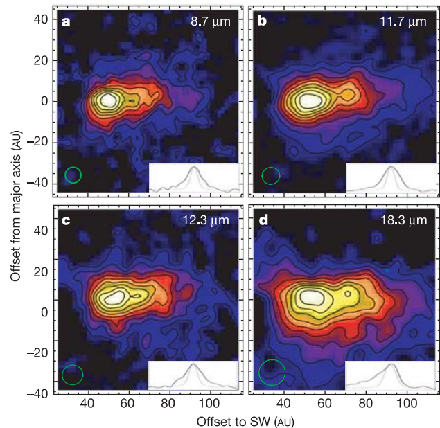
Figure 3 The residual emission. Images result from subtracting the NE wing from the SW wing along lines through the star. The nine evenly spaced contour levels are at the 10, 20, 30, 40, 50, 60, 70, 80 and 90% peak values of 0.228, 0.321, 0.335 and 0.527 mJy pixel ^{-1} at 8.7, 11.7, 12.3 and 18.3 \mu\text{m} , respectively. Corresponding peak signal-to-noise ratios are 27, 48, 24 and 15, respectively. The 24.6- \mu\text{m} residual is not shown, because features are ambiguous. PSF FWHM contours are in the lower left corners. Each inset shows a minor-axis scan (with the displayed linear scale compressed by a factor of two) through the peak (NW to right, SE to left) and the normalized PSF.
