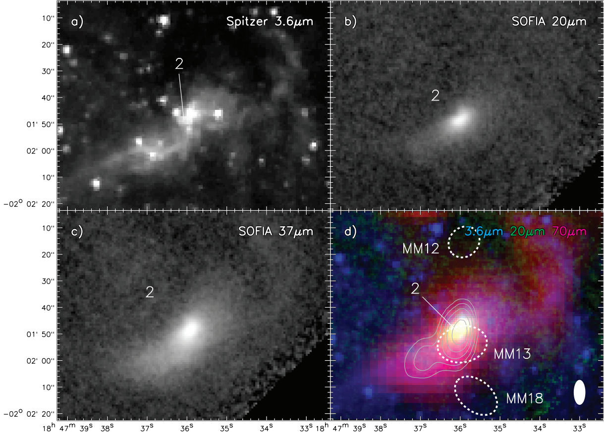
Figure 19. Images of the MM13 region containing infrared source 2, with (a) Spitzer 3.6\,\mu\text{m} , (b) SOFIA 20\,\mu\text{m} , (c) SOFIA 37\,\mu\text{m} , and (d) a three-color RGB image made from Herschel 70\,\mu\text{m} (red), SOFIA 20\,\mu\text{m} (green), and Spitzer 3.6\,\mu\text{m} (blue). In panel (d), the dashed white ellipses denote the 2D Gaussian size and position of the mm fragment MM13, as well as nearby MM12 and MM18 (from Motte et al. 2003 ). Contours are 6 cm radio continuum emission from Urquhart et al. (2009) , and the filled ellipse on the bottom right corner shows the radio beam size and shape.
