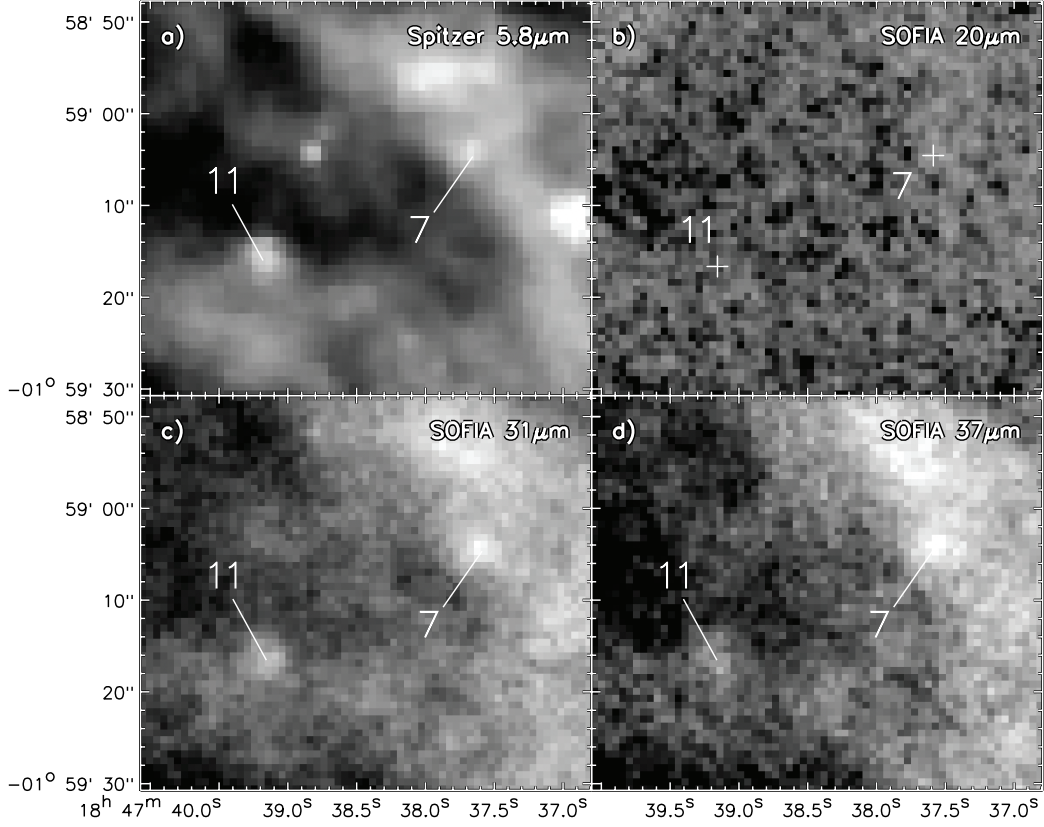
Figure 20. Images of the region containing infrared sources 7 and 11, with (a) Spitzer 5.8\,\mu\text{m} , (b) SOFIA 20\,\mu\text{m} , (c) SOFIA 31\,\mu\text{m} , and (d) SOFIA 37\,\mu\text{m} . In all panels the infrared sources are labeled numerically, but source positions marked by a cross are undetected at that wavelength.
