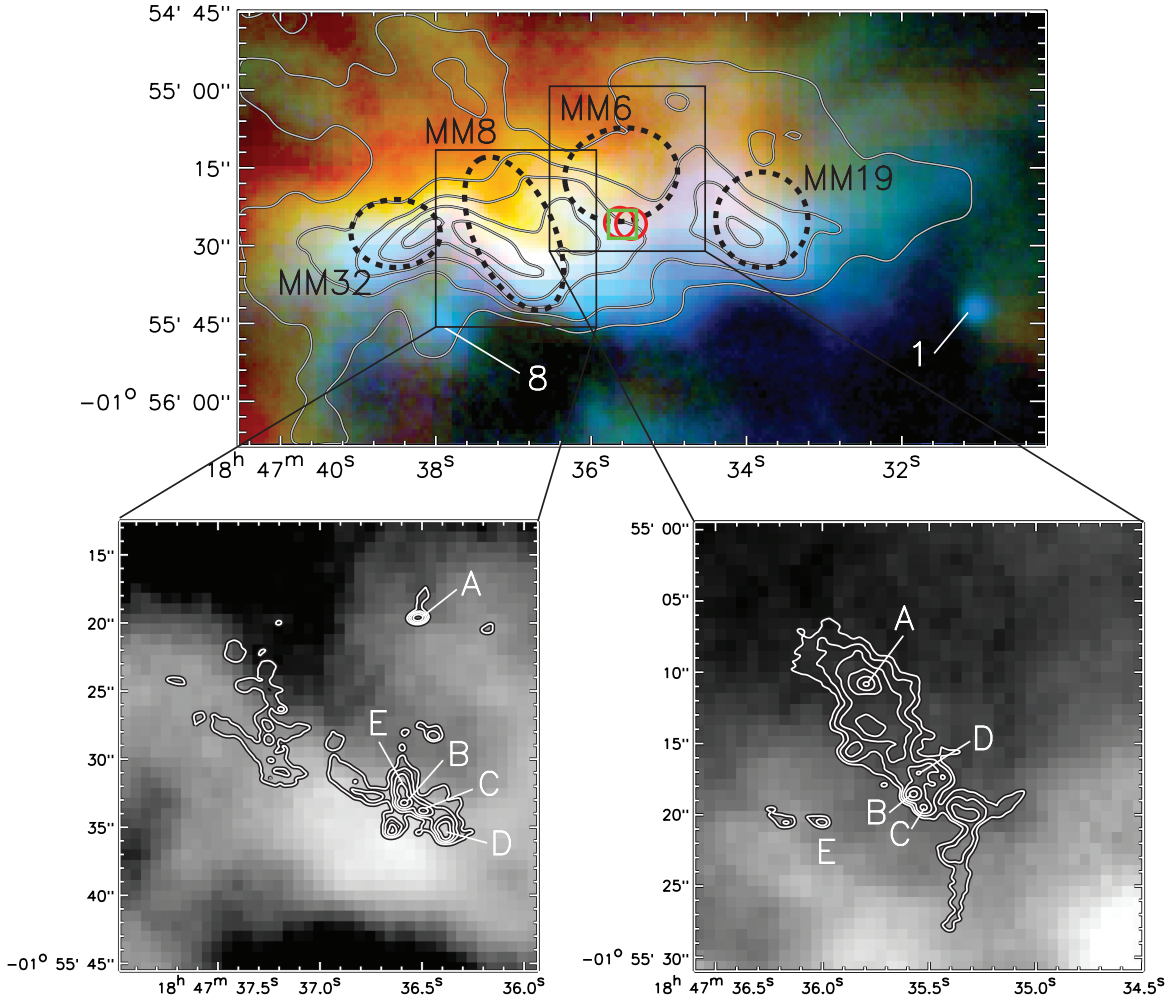
Figure 18. (Top) Three-color RGB image of the MM6 & MM8 ridge from Figure 17 overlaid with contours from the 6 cm data from the VLA archive with 4.5'' resolution. White numerical labels indicate the location and name of the mid-infrared sources. The dashed black ellipses denote the 2D Gaussian sizes and positions of the mm fragments MM6, MM8, MM19, and MM32 defined by Motte et al. (2003). Small red circles mark the locations of the water masers from Valdetarro et al. (2001) and Han et al. (1998), though they have \sim 20'' positional uncertainty. The green square marks the location of the 5 cm OH maser from Baudry et al. (1997) which has 65'' uncertainty. (Bottom-Left) Closeup 20\,\mu\text{m} image of the region around MM8, with the 1.3 mm map of MM8 from Cortes et al. (2019) overlaid as contours, with individual mm cores labeled as letters. (Bottom-Right) Closeup 20\,\mu\text{m} image of the region around MM6, with the 1.3 mm contours of MM6 from Cortes et al. (2019).
