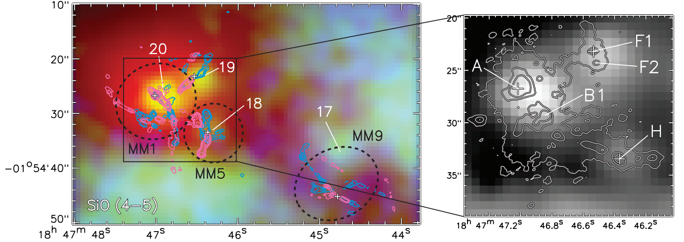
Figure 10. (Left) The same 3-color image of the MM1 region as shown in Figure 9 overlaid with the SiO (4–5) outflow contours from Nony et al. (2020). Light blue contours denote blue-shifted outflow velocities, and light red contours denote red-shifted velocities. The dashed black ellipses denote the 2D Gaussian sizes of the millimeter fragments with names given by Motte et al. (2003). The white crosses (in both images) denote the mm core locations thought to be at the center of the outflows. (Right) A zoomed in area on the region around mid-infrared sources 18, 19, and 20 at 31\,\mu\text{m} . White contours are the high-resolution ( 0.44'' ) 1.3\,\text{mm} emission showing the individual cores from Motte et al. (2018). Alphabetical labels of the mm cores from Cortes et al. (2016).
