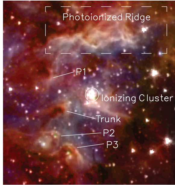
Figure 22. Large scale infrared features of W43 Main. Labeled are the locations of the photoionized ridge north of (and heated/ionized) by the Wolf-Rayet ionizing stellar cluster, which is also labeled. The photoablation of natal cloud material near the ionizing cluster has lead to the appearance of several protuberances (labeled P1, P2, and P3) as well as a trunk-shaped structure. The trunk and protuberances all point back to the ionizing cluster and it may be that the MYSOs seen in projection coincident with P2 and P3 are actually contained within the protuberances. This image is the same 4-color image as in Figure 1, but with higher contrast to show detail.
