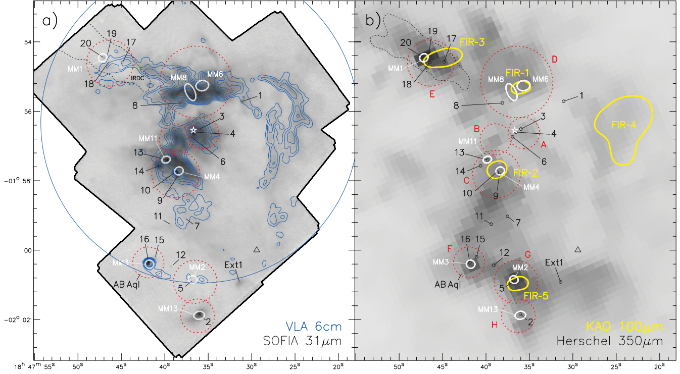
Figure 6. Multi-wavelength comparisons of W43 Main. a) The SOFIA 31\,\mu\text{m} image overlaid with VLA 6\,\text{cm} archival data contours (with 4.6'' resolution) in dark blue showing the spatial similarities in wide-spread ionized gas and warm dust emission. The large dark blue circle shows the field of view of this radio continuum image, which does not extend as far south as the SOFIA data. b) The Herschel 350\,\mu\text{m} image showing the spatial distribution of the cold dust. Overlaid in yellow is the brightest contour for each source from the KAO 100\,\mu\text{m} image from Lester et al. (1985) , with 100\,\mu\text{m} source names also labeled in yellow. In both panels of this figure, we give the locations of the SOFIA compact sources in black, as well as the locations and 2-dimensional FWHM sizes of several millimeter cloud fragments from Motte et al. (2003) , which are shown as white ellipses with their names labeled in white. Also shown in both panels is a white star marking the center of the WR/OB stellar cluster. The area contained within the dashed black lines in the upper left of both panels is an infrared dark cloud (IRDC). The triangle symbol shows the location of the MYSO candidate of Saral et al. (2017) , though we do not detect this source at any SOFIA wavelength. The red dotted circles and red labels mark the identified mid-infrared sub-regions from this work used in the evolutionary analyses, with the circles representing the size of the apertures used for photometry (see Sections 5.4 and 5.5).
