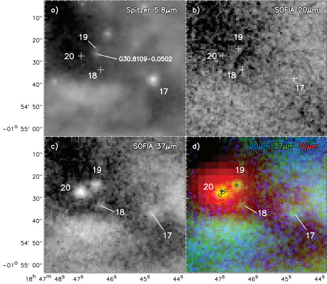
Figure 9. Images of the MM1 region containing infrared sources 17-20, with (a) Spitzer 5.8\mu\text{m} , (b) SOFIA 20\mu\text{m} , and (c) SOFIA 37\mu\text{m} . In panel (d), the region is shown as a three-color infrared composite and black crosses mark the positions of 6.7 GHz methanol masers from Nguyen et al. (2022) , and black circles mark the locations of OH masers from Beuther et al. (2019) . In all panels the infrared sources are labeled numerically, but source positions marked by a cross are undetected at that wavelength.
