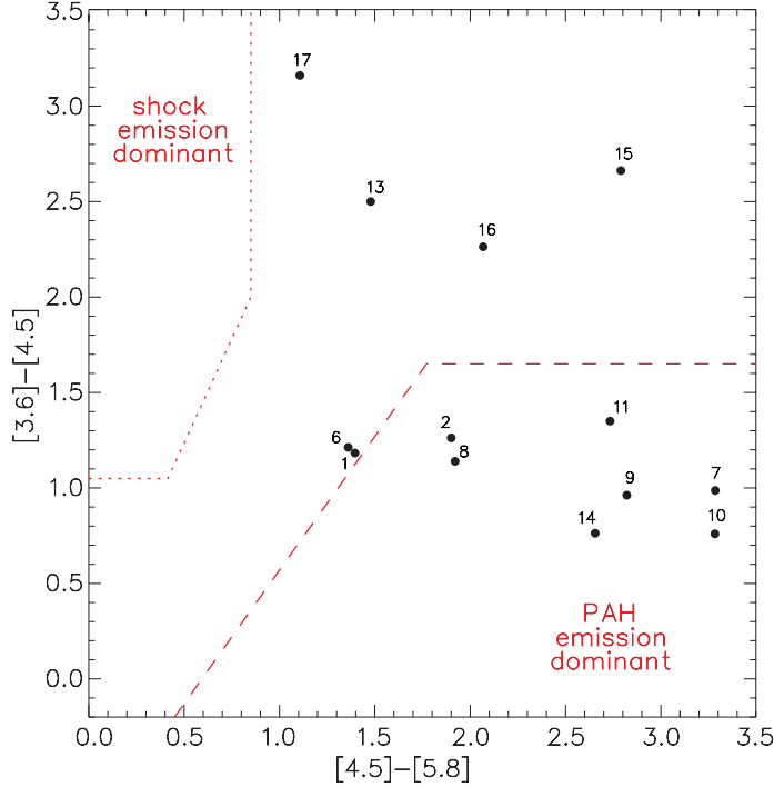
Figure 7. A color-color diagram for compact sources in W43 Main utilizing our background-subtracted Spitzer-IRAC 3.6, 4.5, and 5.8\mu\text{m} source photometry to distinguish “shocked emission dominant” and “PAH emission dominant” YSO candidates from our list of compact sub-components. Above (up-left) the dotted line indicates shock emission dominant regime. Below (bottom-right) the dashed line indicates PAH dominant regime. We adopt this metric from Gutermuth et al. (2009) . Some sources are not included in this diagram due to non-detection or saturation in the Spitzer-IRAC bands.
