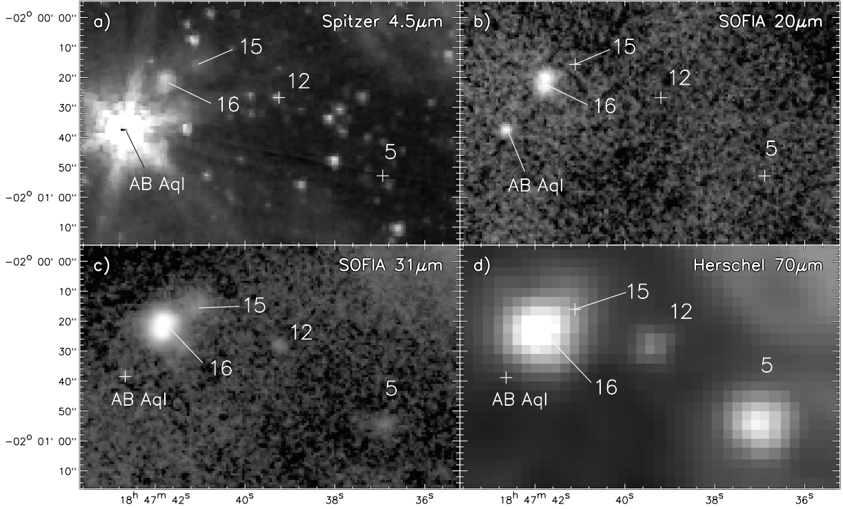
Figure 11. Images of the MM2 & MM3 region containing infrared sources 5, 12, 15 and 16, with (a) Spitzer 4.5\,\mu\text{m} , (b) SOFIA 20\,\mu\text{m} , (c) SOFIA 31\,\mu\text{m} , and (d) Herschel 70\,\mu\text{m} . In all panels the infrared sources are labeled numerically, but source positions marked by a cross are undetected at that wavelength.
