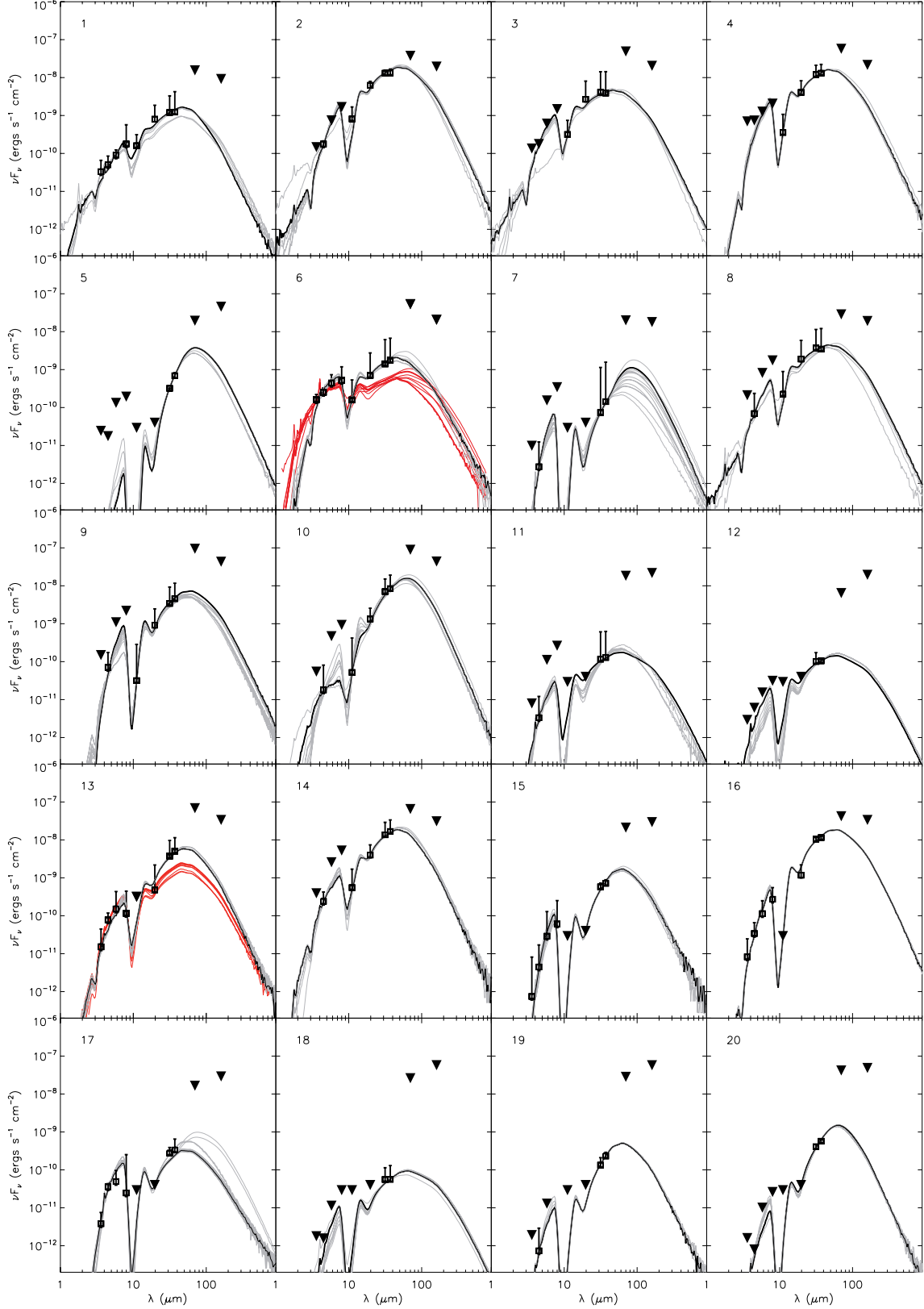
Figure 8. SED fitting with ZT MYSO SED models for compact sources in W43 Main. Black lines are the best fit model to the SEDs, and the system of gray lines are the remaining fits in the group of best fits (from Table 3). Upside-down triangles are data that are used as upper limits in the SED fits. For Sources 6 and 13 only, the red lines are fits using the nominal upper error bars, and black/gray lines are fits use upper errors matched to the lower errors.
