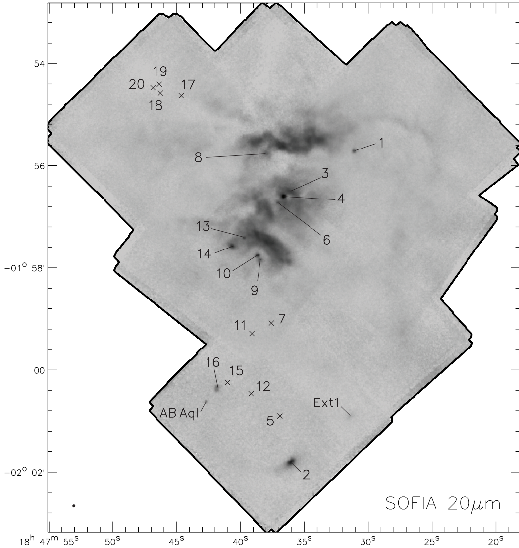
Figure 3. W43 Main image mosaic taken at 20\,\mu\text{m} by SOFIA shown in inverse color (i.e. brighter features are darker in color). See Figure 2 caption for further information.
