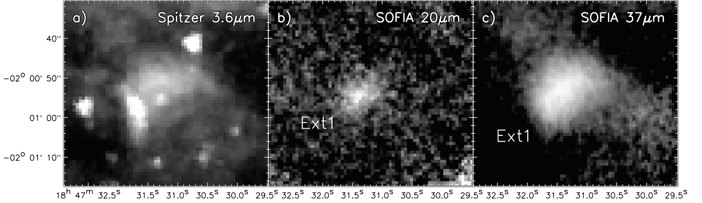
Figure 21. Images of infrared source Ext1 at (a) Spitzer 3.6\,\mu\text{m} , (b) SOFIA 20\,\mu\text{m} , and (c) SOFIA 37\,\mu\text{m} .
