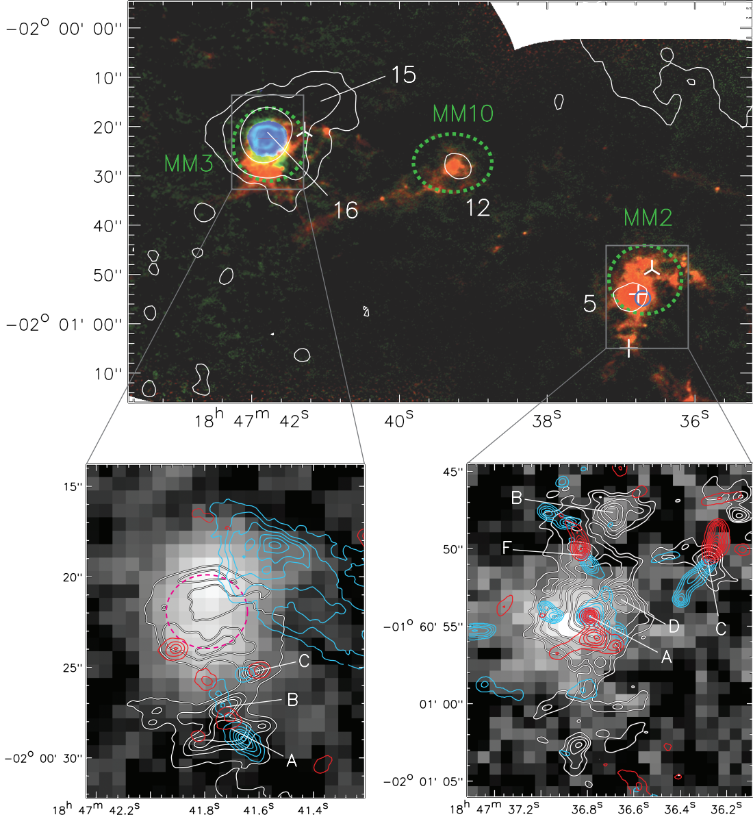
Figure 12. (Top) Three-color RGB image of the MM2 & MM3 region from Pouteau et al. (2022) showing cold dust continuum at ALMA 1.3 mm (green) and 3 mm (red). Free-free emission at H41 \alpha recombination line (blue) show the location of the UCH II region. White contours are from the SOFIA 31 \mu\text{m} emission. The dashed green ellipses denote the 2D Gaussian sizes and positions of the mm fragments MM2, MM3, and MM10 defined by Motte et al. (2003). White numerical labels are given for the mid-infrared sources identified in this present work. White upside-down ‘Y’ symbols mark the locations of the Class I methanol masers (from Yang et al. 2017), white crosses mark the locations of the center of the Class II methanol maser emission (from Nguyen et al. 2022), and the blue circle symbol marks the location of the center of the hydroxyl maser emission (from Beuther et al. 2019). (Bottom-Left) The SOFIA 20 \mu\text{m} image of mid-infrared source 16, with 1.3 mm contours of Cortes et al. (2019) with the brightest mm cores labeled. The magenta ellipse traces the donut-shaped mm shell discussed in the text. (Bottom-Right) The SOFIA 31 \mu\text{m} image of mid-infrared source 5, with 1.3 mm contours of Cortes et al. (2019) with the brightest mm cores labeled. In both bottom panels the red and blue contours are the red- and blue-shifted CO outflow emission from Nony et al. (2023).
