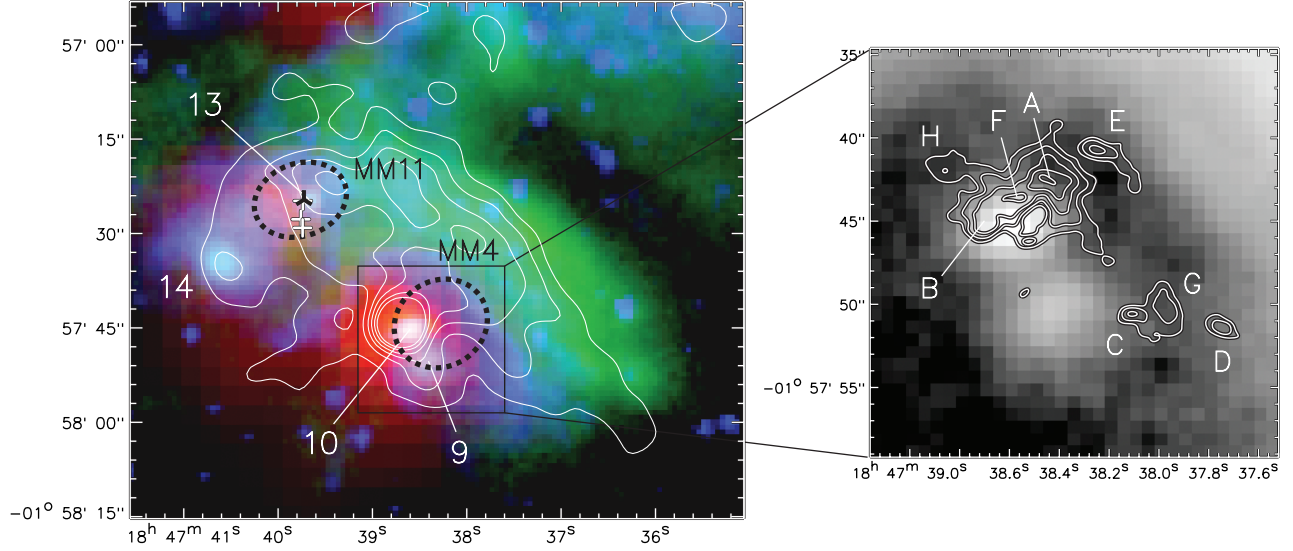
Figure 14. (Left) Three-color RGB image of the MM4 and MM11 region (from Figure 13), overlaid with contours from the 6 cm data from the VLA archive with 4.5'' resolution. The dashed black ellipses denote the 2D Gaussian sizes and positions of the mm fragments MM4 and MM11 defined by Motte et al. (2003). White numerical labels are given for the mid-infrared sources identified in this present work. White crosses mark the locations of the center of the Class II methanol maser emission (from Walsh et al. 1998; Hu et al. 2016; Reid et al. 2019), and the black upside-down ‘Y’ symbol marks the locations of the Class I methanol maser (from Nguyen et al. 2022). (Right) Closeup 20\,\mu\text{m} image of the region around sources 9 and 10, with the 1.3 mm map of MM4 from Cortes et al. (2019), with individual mm cores labeled as letters.
