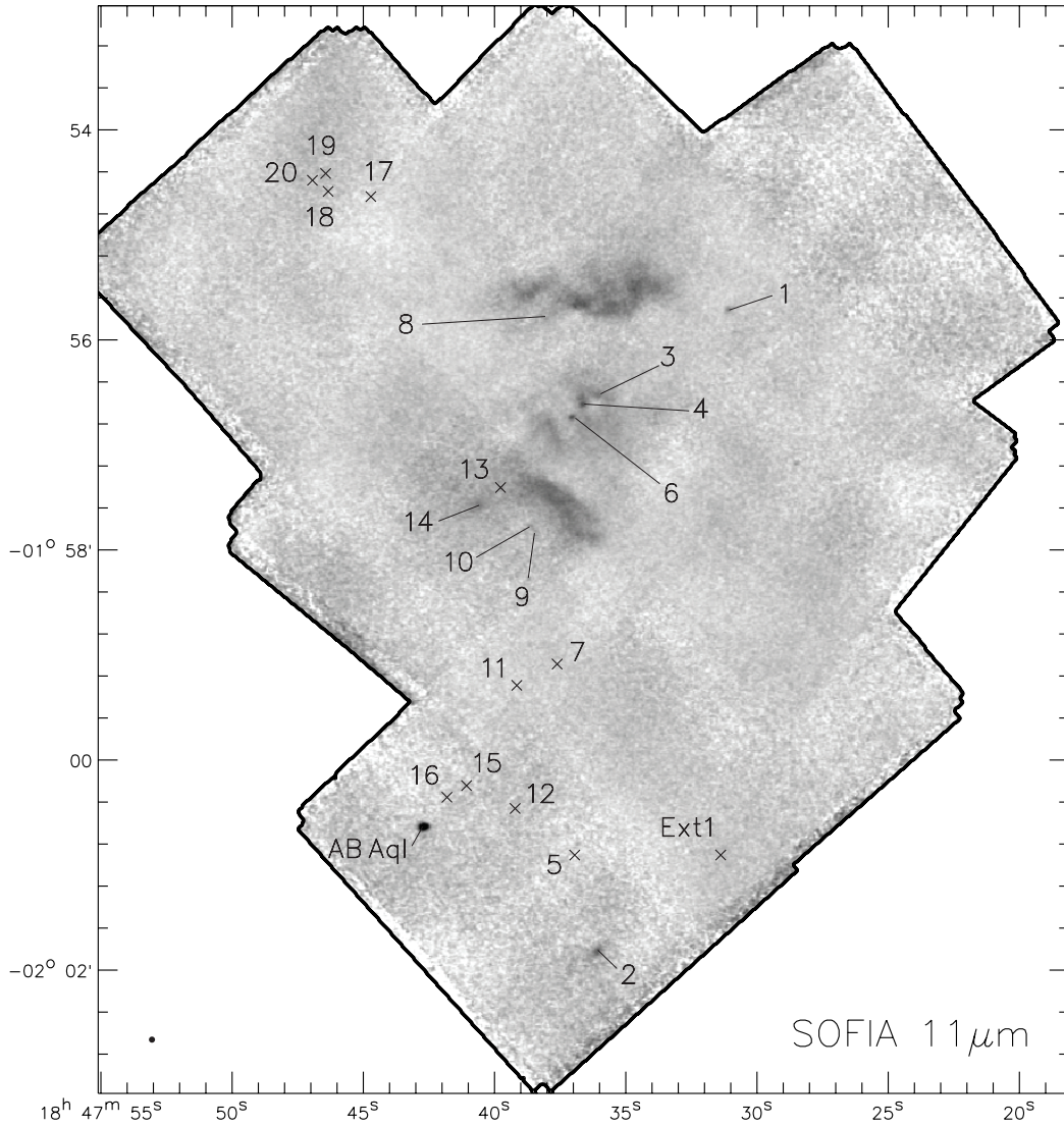
Figure 2. W43 Main image mosaic taken at 11\,\mu\text{m} by SOFIA shown in inverse color (i.e. brighter features are darker in color). Sources labeled with numbers are the mid-infrared compact sources identified in this work. The positions of the mid-infrared sources marked with an 'x' are not seen at this wavelength. The small black dot in the lower left indicates the resolution of the image at this wavelength.
