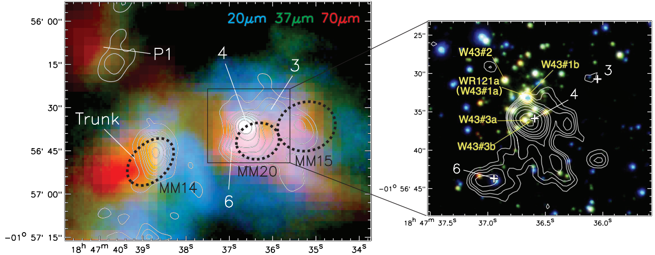
Figure 16. (Left) Three-color RGB image of the central W43 Main region with Herschel 70 \mu\text{m} (red), SOFIA 37 \mu\text{m} (green), and SOFIA 20 \mu\text{m} (blue), overlaid with contours from the 6 cm data from the VLA archive with 4.5'' resolution. White numerical labels indicate the location and name of the mid-infrared sources. The dashed black ellipses denote the 2D Gaussian sizes and positions of the mm fragments MM14, MM15, and MM20 defined by Motte et al. (2003). (Right) A 3-color image of the W43 stellar cluster made with ESO VLT J, H, and Ks bands in blue, green, and red color, respectively (adapted from Luque-Escamilla et al. 2011). Contours are from VLA 6 cm data taken in its extended B-configuration with \sim 1.5'' resolution. Yellow labels show the WR/OB cluster members identified by Blum et al. (1999) and Luque-Escamilla et al. (2011) in the near-infrared. White crosses indicate the locations of the mid-infrared source peaks at 37 \mu\text{m} .
