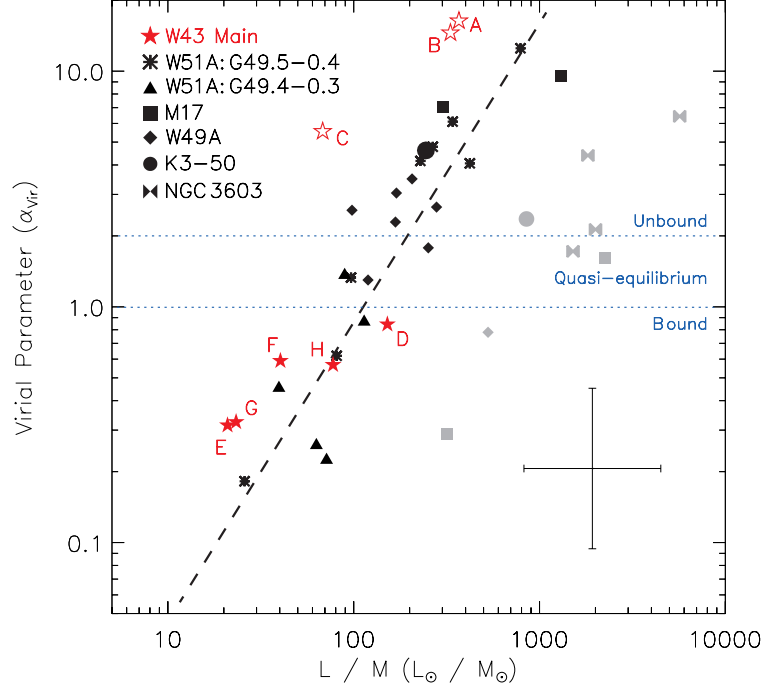
Figure 23. Virial parameter ( \alpha_{\text{vir}} ) vs. L/M of all infrared sub-regions in all GH II regions studied so far, with values for the sub-regions of W43 Main given in Table 4 plotted as red stars with red labels (see also Figure 6). The open star symbols mean that we are less confident in the results due to unresolved spectroscopic feature blending. Asterisks are values for the sub-regions in W51A:G49.5-0.4 with triangles for the sub-regions in W51A:G49.4-0.3. The dashed line indicates the best line fit from Paper I to both W51A GH II regions only (slope \sim 1.28 in log-space). Squares show the sub-regions of M17, diamonds show the data for the sub-regions in W49A, the filled circles are for K3-50, and the bowtie symbols are for NGC 3603. Gray symbols indicate sources that have significantly higher L/M values that place them to the right of the main trend, and may have significant contamination from external heating/ionization. Objects to the lower left are evolutionarily younger, and sources to the upper right, older. Sources above the blue dotted line at \alpha_{\text{vir}} = 2 , are gravitationally unbound and expanding, and all source below the blue dotted line at \alpha_{\text{vir}} = 1 , are self-gravitationally bound and collapsing. Sources in the region between the blue dotted lines ( 1 < \alpha_{\text{vir}} \leq 2 ) are in quasivirial equilibrium, meaning the clump is slightly expanding but still gravitationally bound. The error bar at the bottom left shows the typical uncertainty (a factor of \sim 2 ) in both L/M and \alpha_{\text{vir}} .
