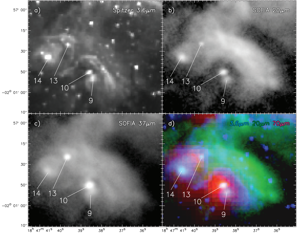
Figure 13. Images of the MM4 and MM11 region containing infrared sources 9, 10, 13 and 14, with (a) Spitzer 3.6\,\mu\text{m} , (b) SOFIA 20\,\mu\text{m} , (c) SOFIA 37\,\mu\text{m} , and (d) a three-color RGB image showing cold dust continuum Herschel 70\,\mu\text{m} (red), warm dust at SOFIA 20\,\mu\text{m} (green), and hot dust and photospheric emission at Spitzer 3.6\,\mu\text{m} (blue). In all panels the infrared sources are labeled numerically.
