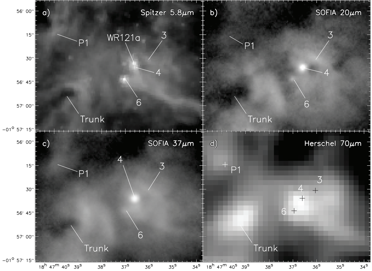
Figure 15. Images of the central W43 Main region containing mid-infrared sources 3, 4, and 6, with (a) Spitzer 5.8\mu\text{m} , (b) SOFIA 20\mu\text{m} , (c) SOFIA 37\mu\text{m} , and (d) Herschel 70\mu\text{m} . Panel a) also shows the position of WR 121a (a.k.a. W43#1a). Also labeled are the protuberance P1 and a photoablated trunk as identified in Figure 22. In all panels the infrared sources are labeled numerically, but source positions marked by a cross are undetected at that wavelength.
