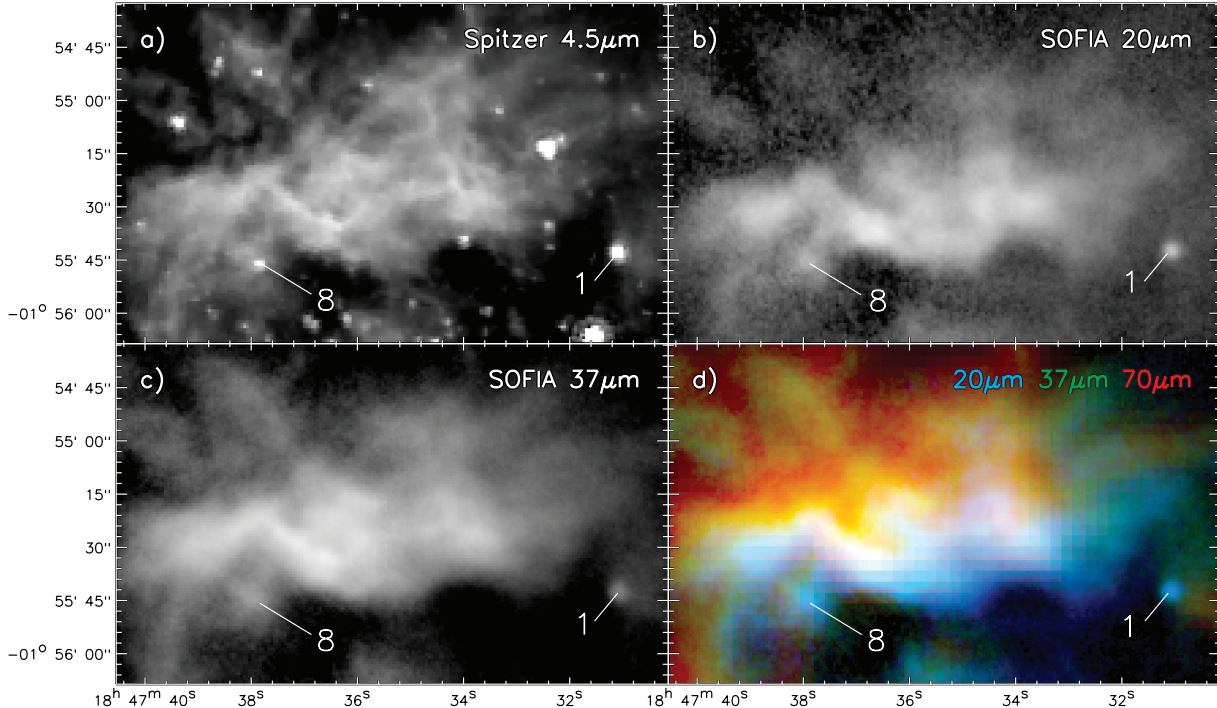
Figure 17. Images of the MM6 & MM8 ridge containing infrared sources 1 and 8, with (a) Spitzer 4.5\mu\text{m} , (b) SOFIA 20\mu\text{m} , (c) SOFIA 37\mu\text{m} , and (d) a three-color RGB image made from Herschel 70\mu\text{m} (red), SOFIA 37\mu\text{m} (green), and SOFIA 20\mu\text{m} (blue) data. In all panels the infrared sources are labeled numerically.
